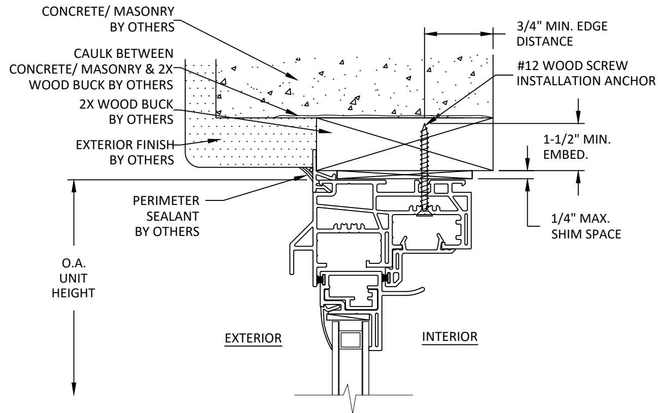
A 3 HEAD SECTION THROUGH FRAME INSTALLATION
